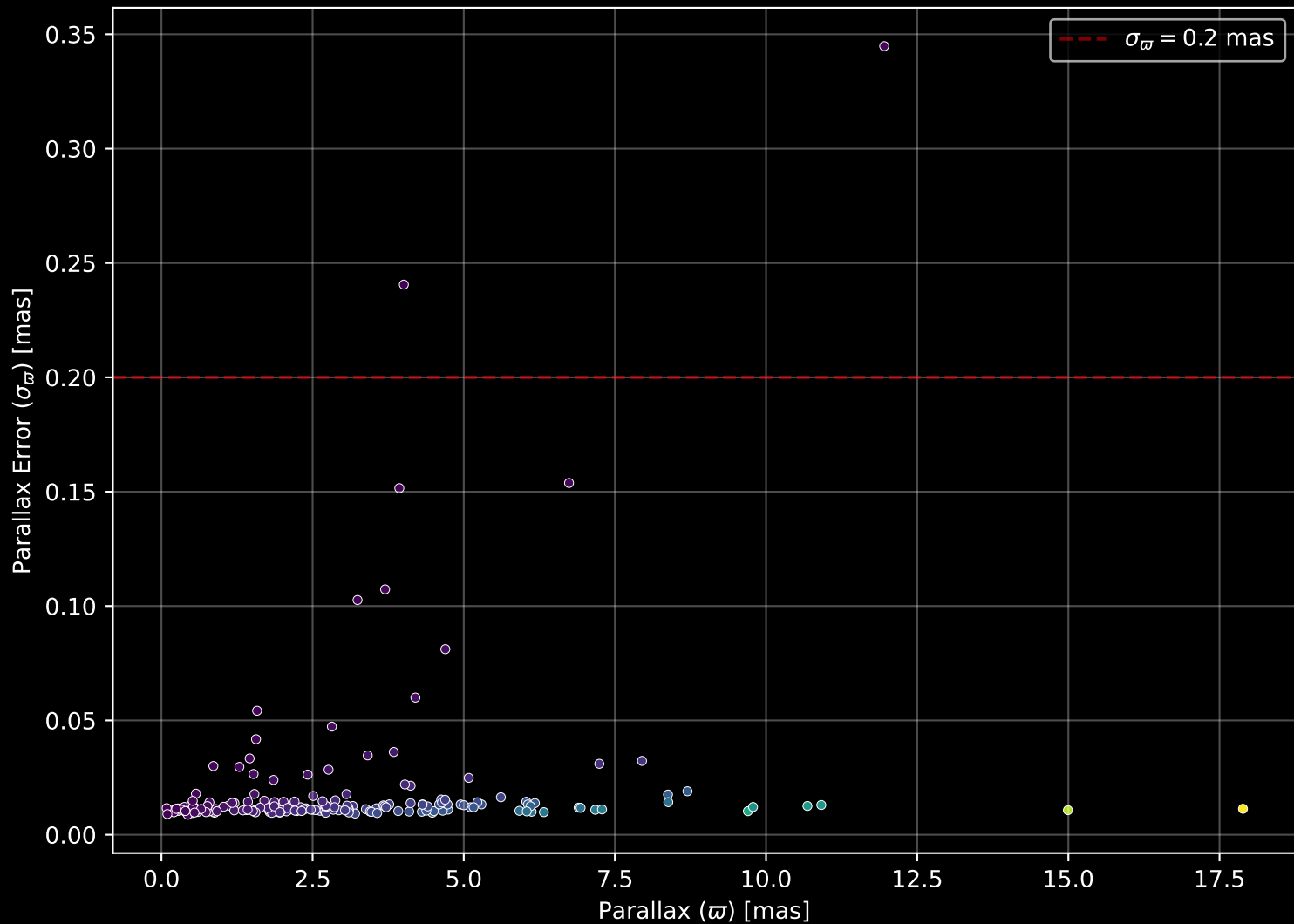
APOGEE DR17 Field: [052+44_MGA] Parallax Quality (n= 185)
