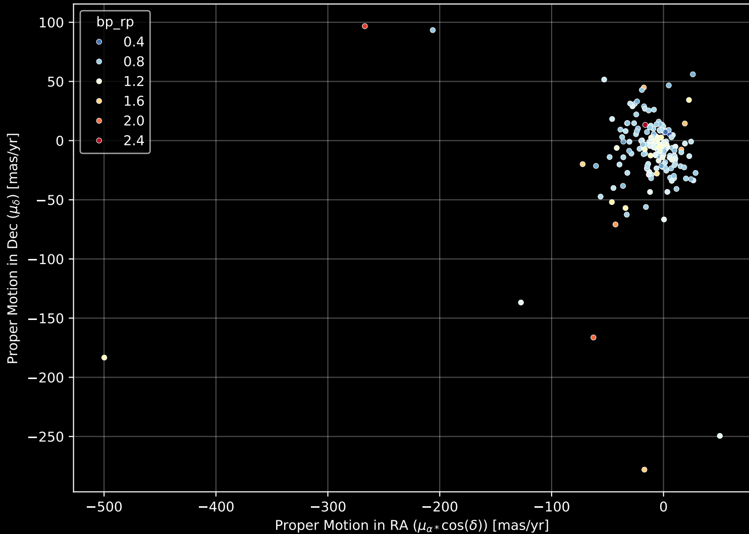
APOGEE DR17 Field: [052+44_MGA] Proper Motion Diagram (n= 185)
