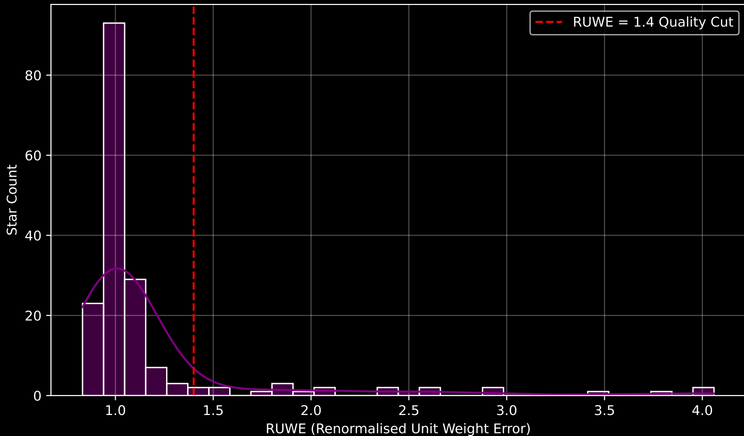
GAPOGEE DR17 Field [052+44_MGA] RUWE Distribution (n= 177)
