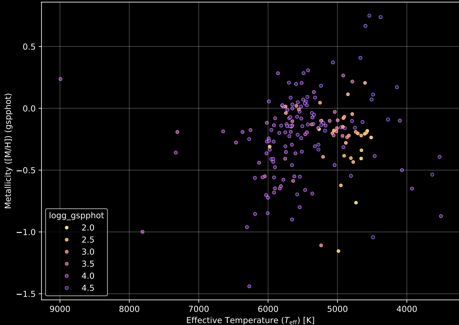
APOGEE DR17 Field: [052+44_MGA] Stellar Population Parameters (n= 185)
