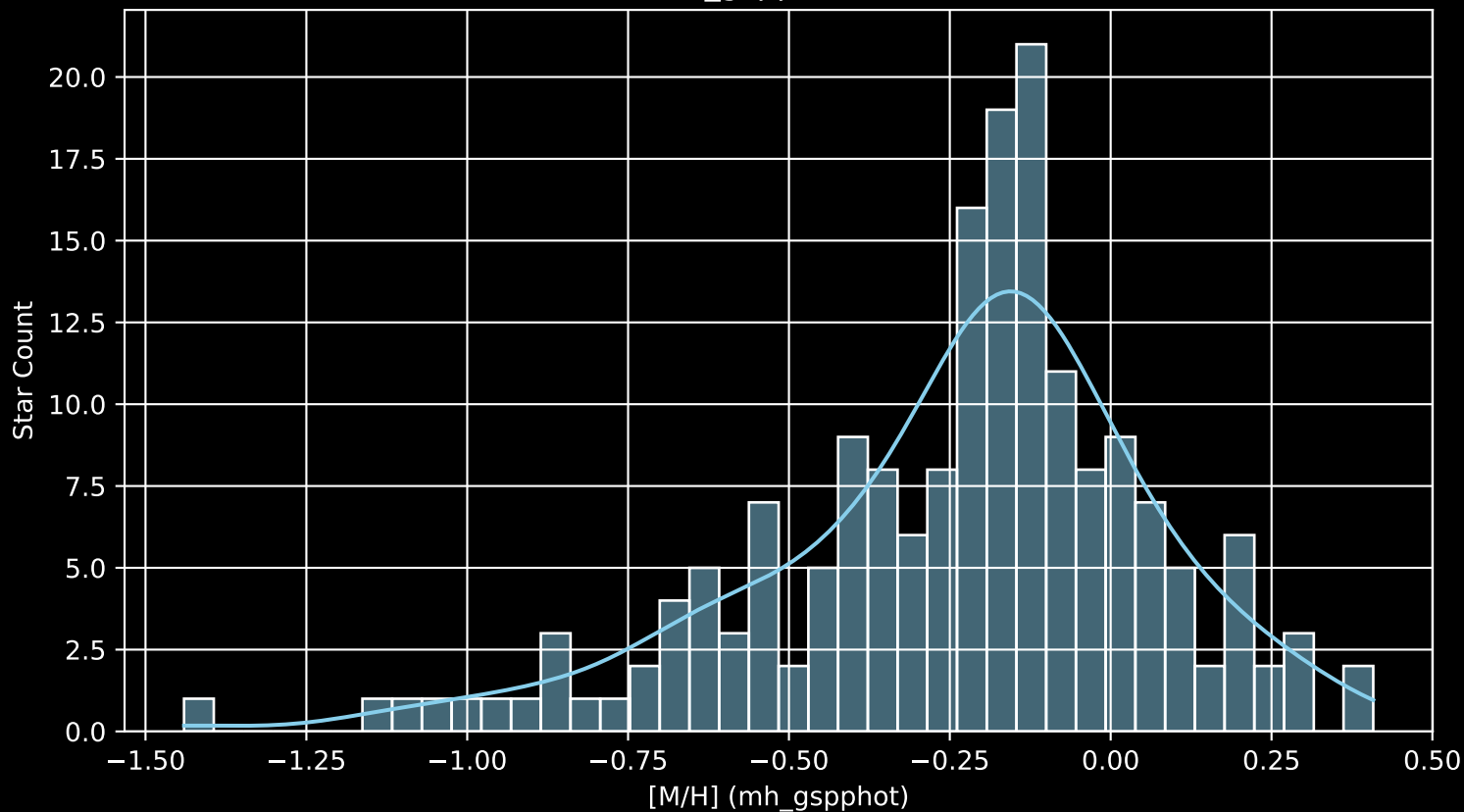
APOGEE DR17 Field: [052+44_MGA [M/H] (mh_gspphot) (n= 182)
