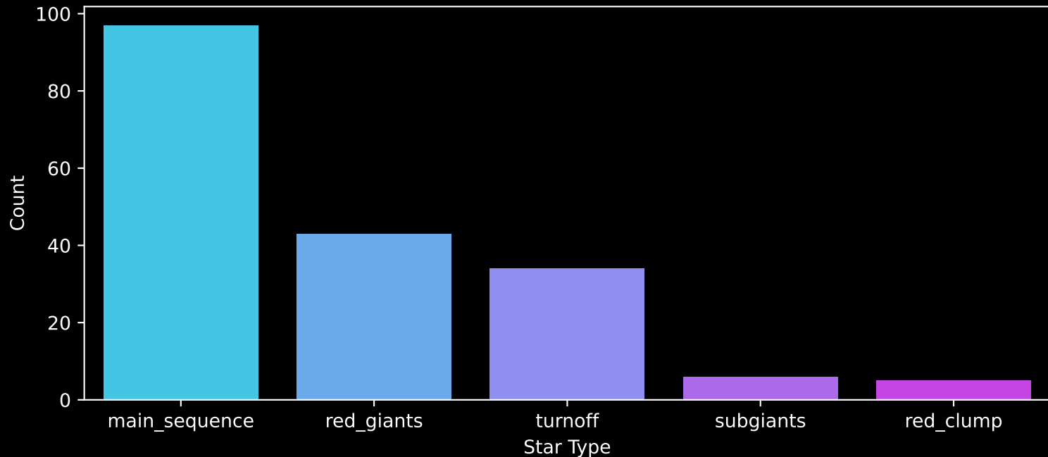
APOGEE DR17 Field: [052+44_MGA] Count plot of Star Type
